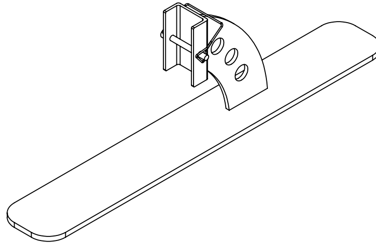
FST150 (with .25 dia wire lock pin)
