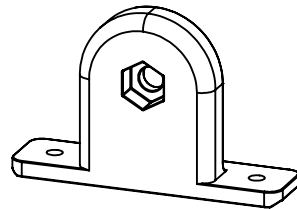
Pivot Base - JPB150
